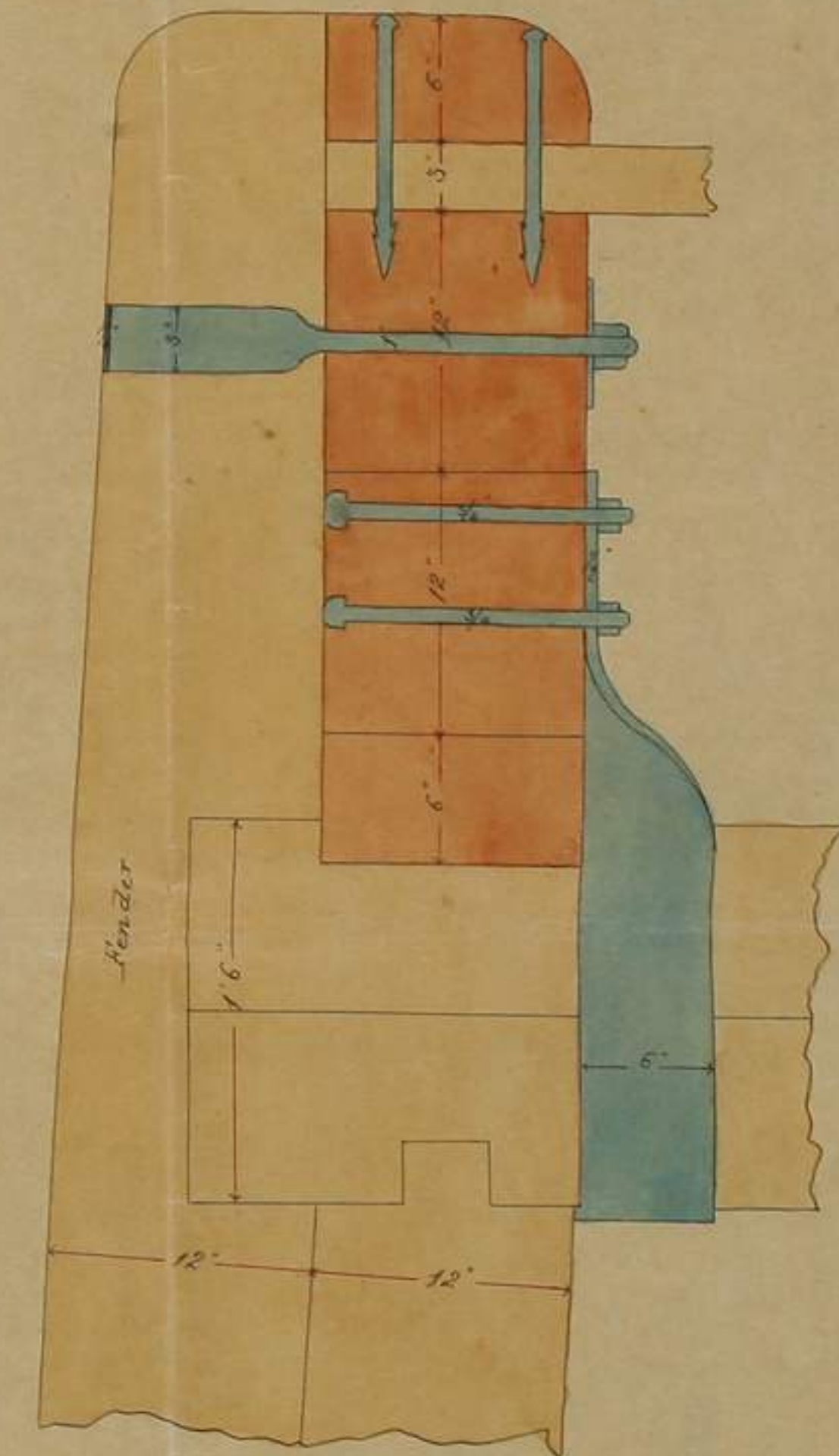
BOTTOM OF FENDERS
