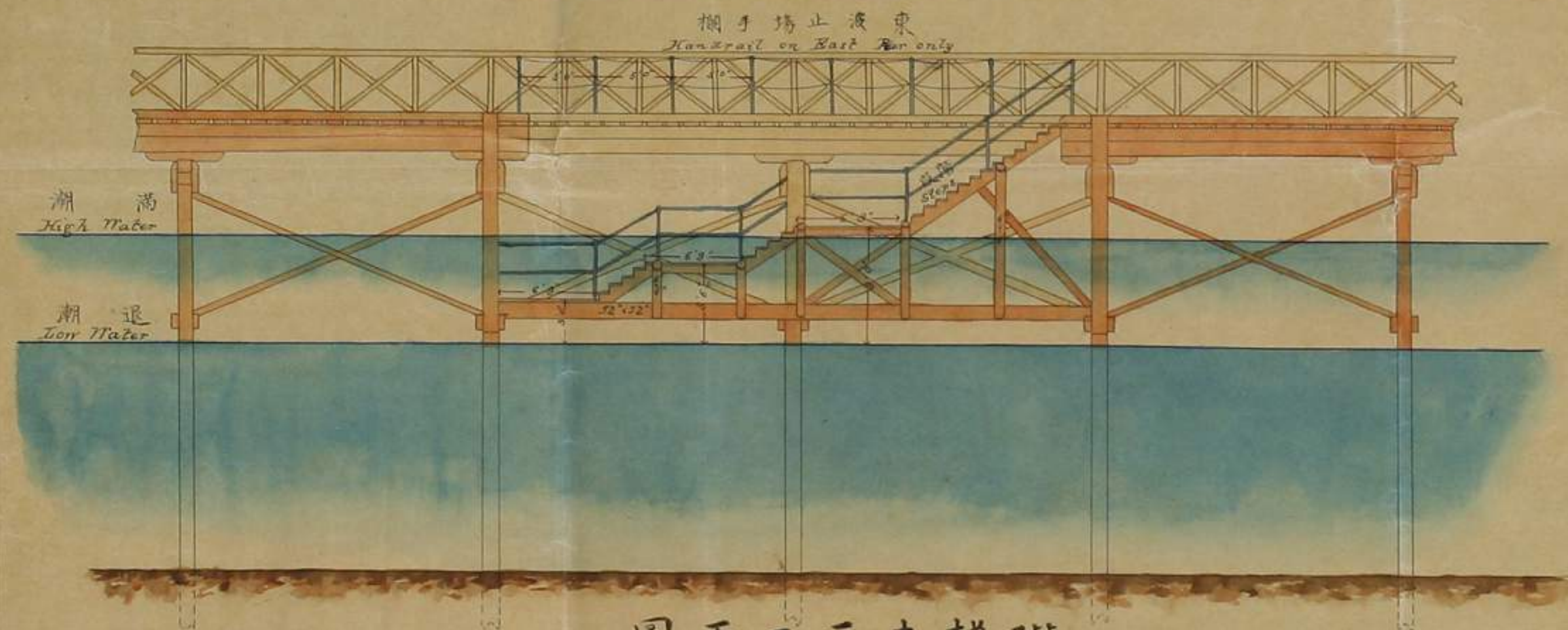
ELEVATION SHEWING STAIR
