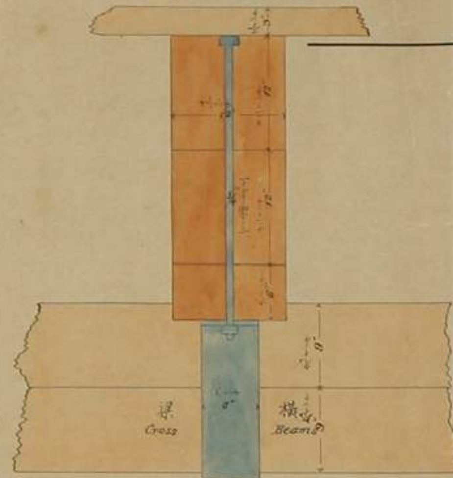
圖截橫 CROSS SECTION
