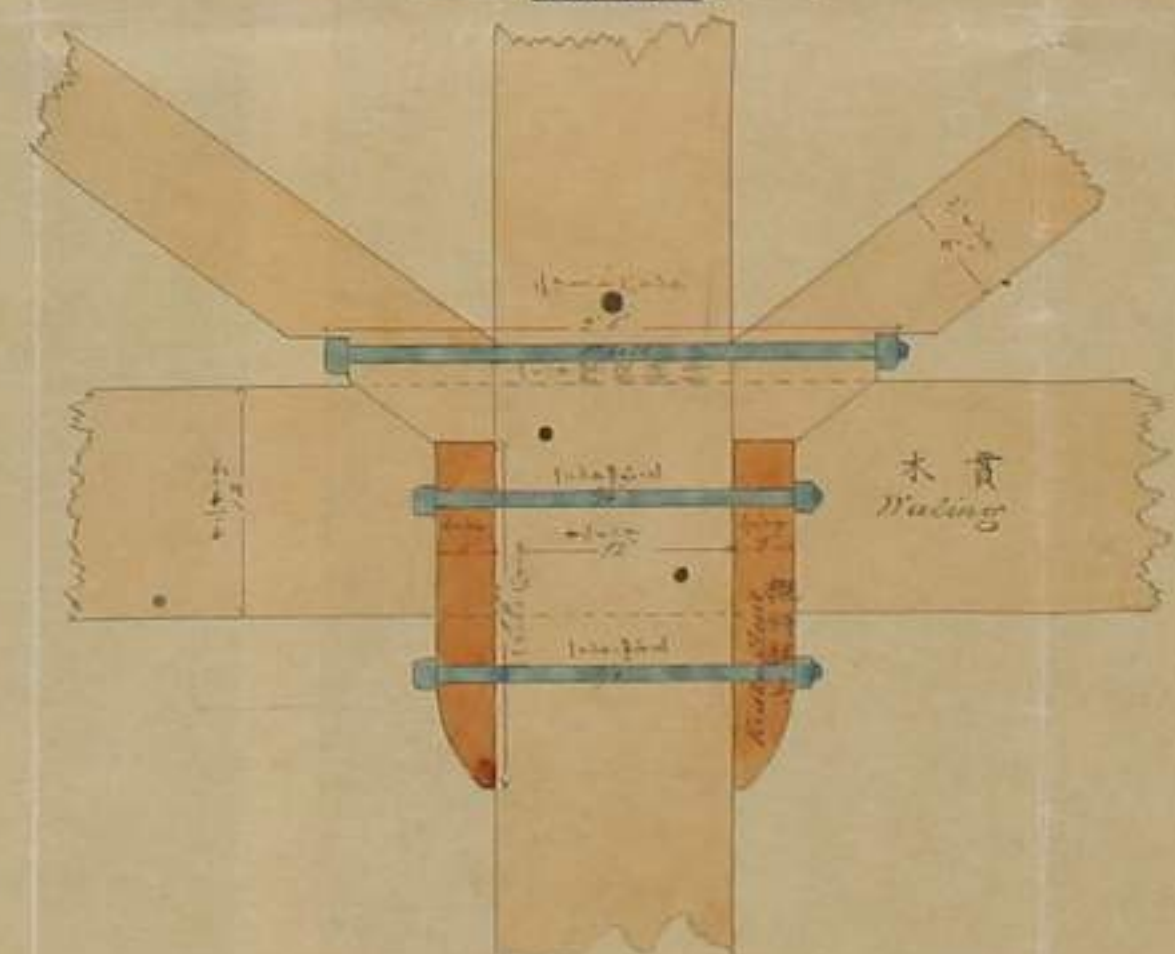
圖截橫 CROSS SECTION
