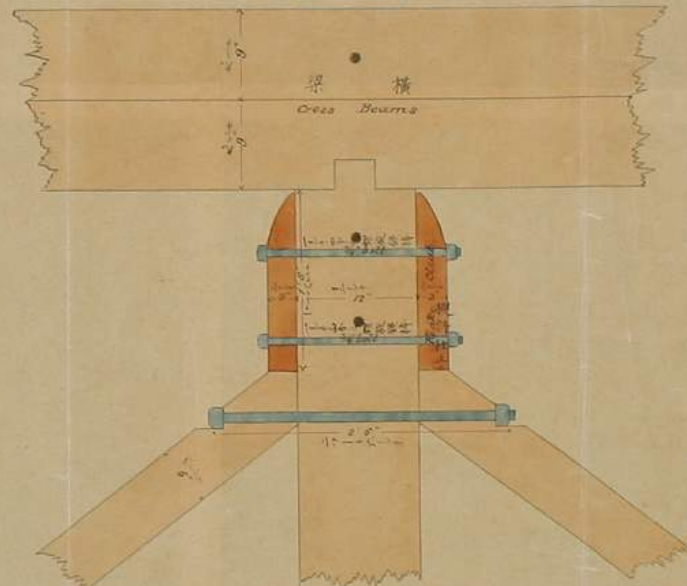
底'架木 BOTTOM OF FRAMEWORK
