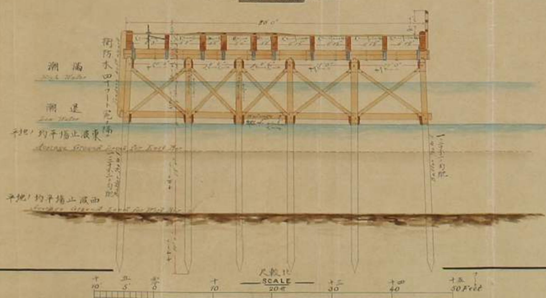
圖截橫 CROSS SECTION
