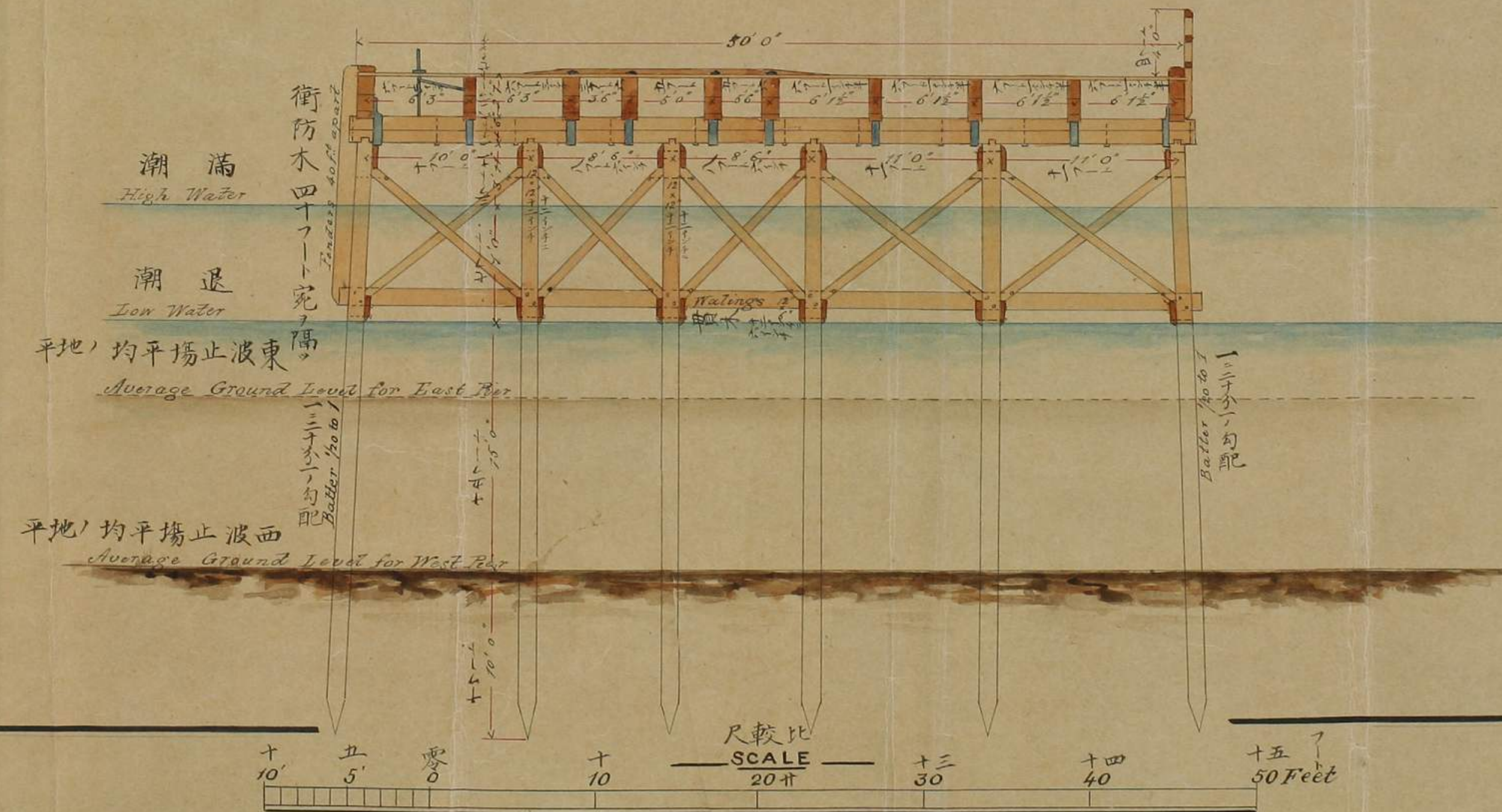
圖截橫 CROSS SECTION
