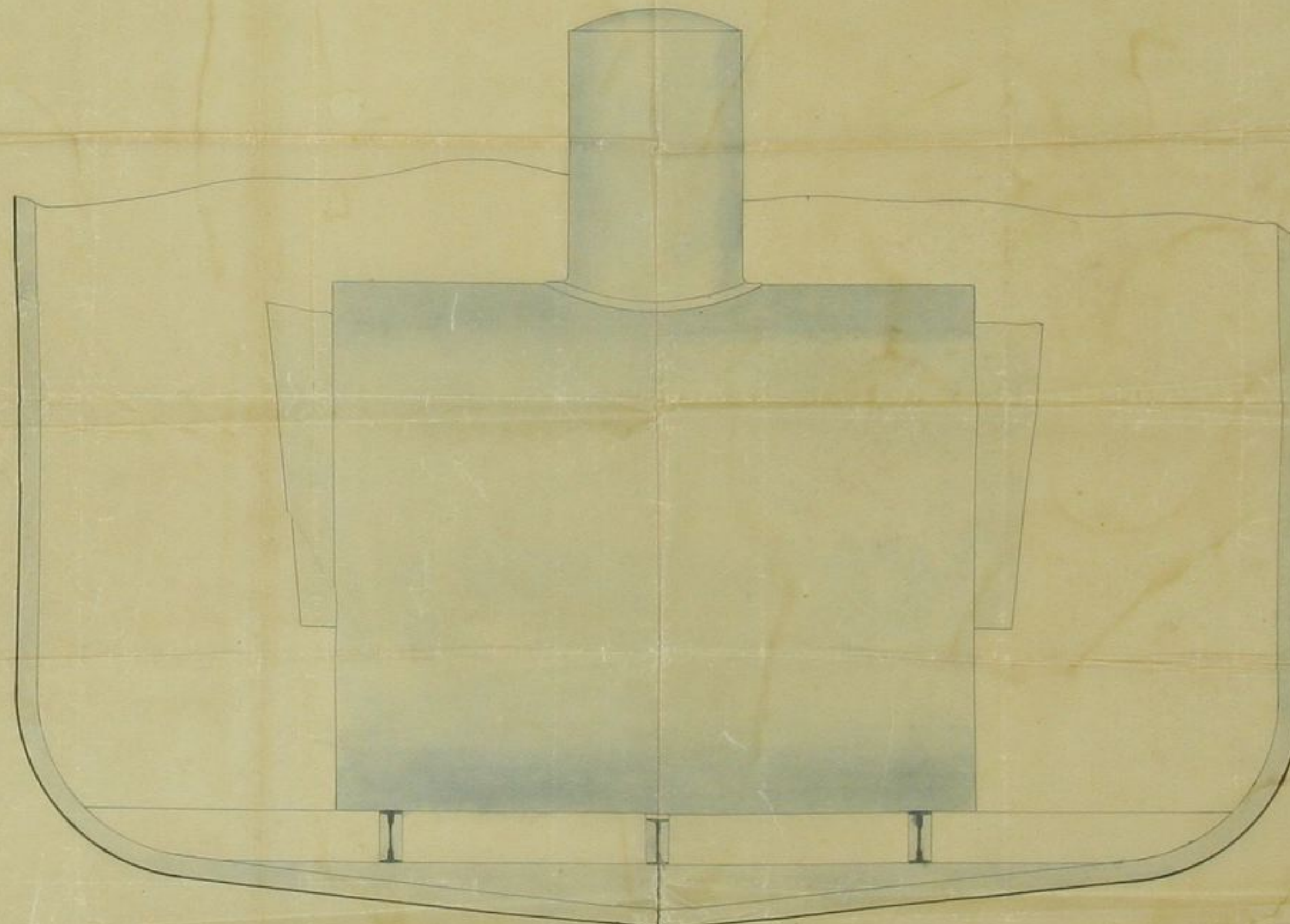
SHIP ARRANGEMENT OF A PAIR OF COMPOUND ENGINES & BOILER CYL s 28" & 50" DIAM s STROKE 2'-2" SCALE 1/2" = A FOOT
