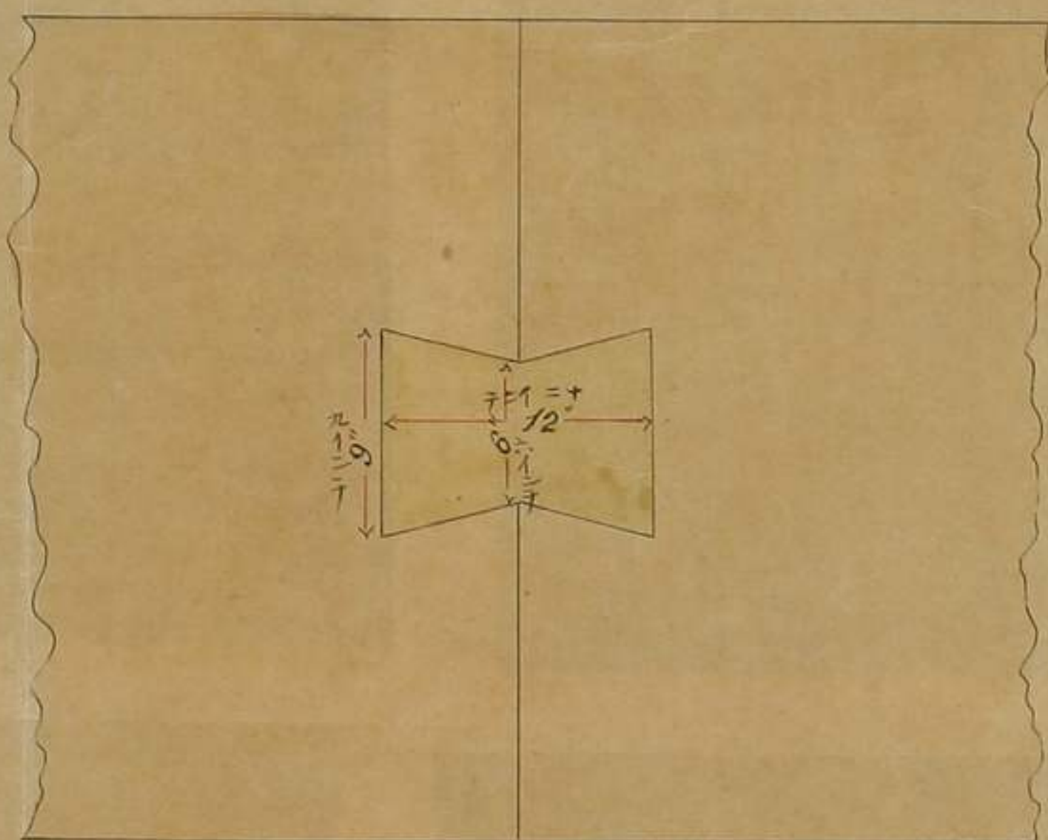
膝ノス合格ヲ石笠 WOODEN JOGGLE AT JOINTS OF COPES
