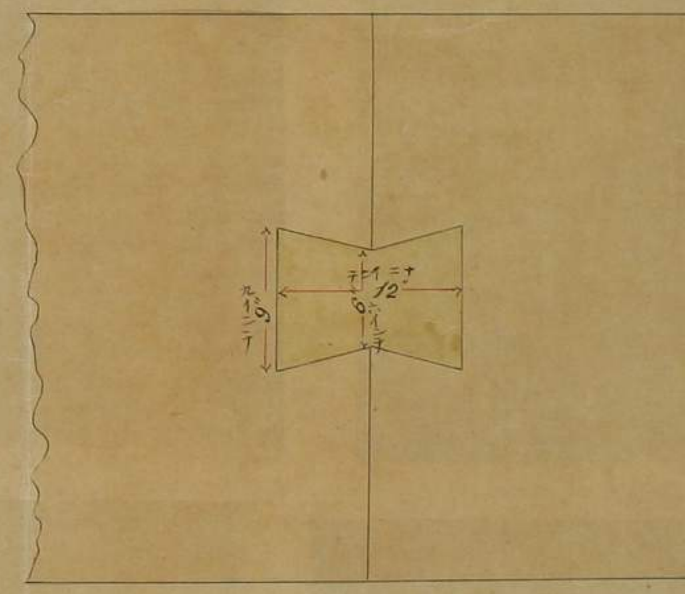
石笪子格合不ル WOODEN JOGGLE AT JOINTS OF COPES
