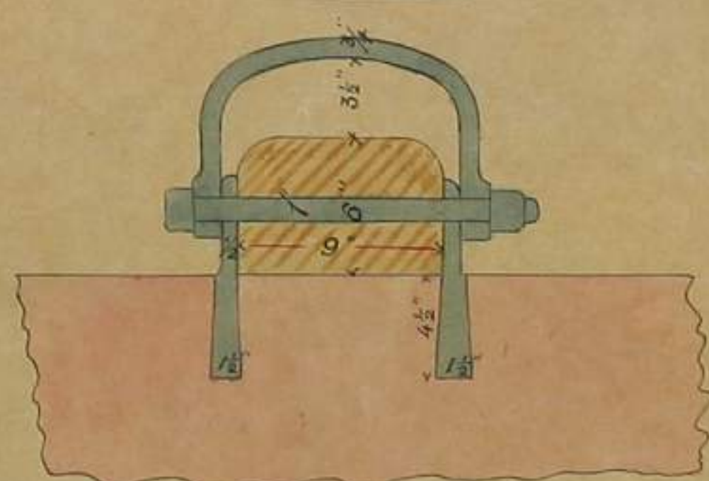
SECTION AT TOP
