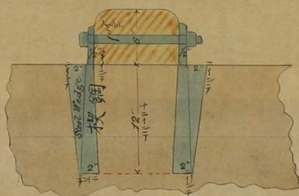
圖斷截ノ底 SECTION AT BOTTOM
