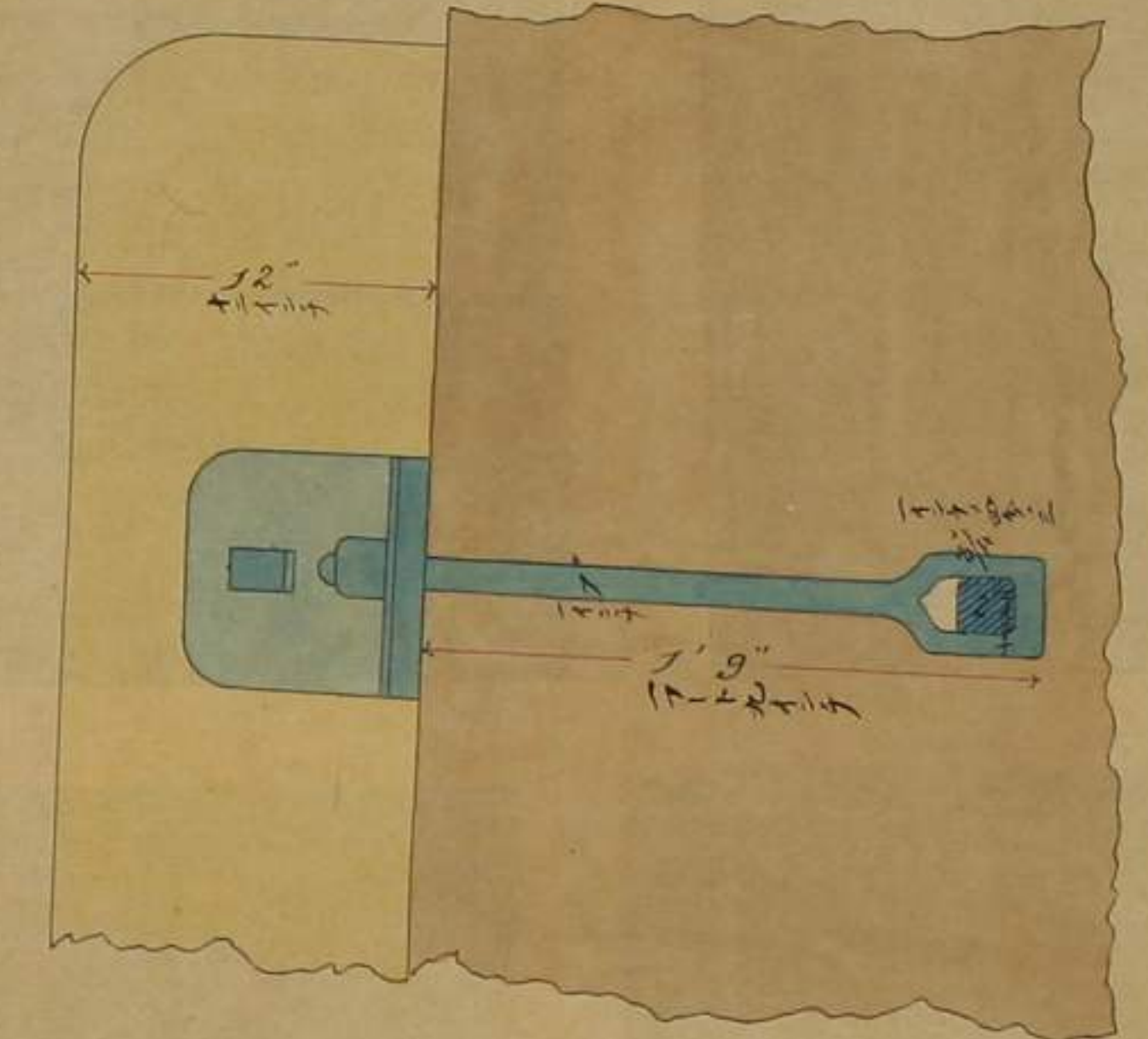
上頂ノ木防衝 FENDERS AT TOP
