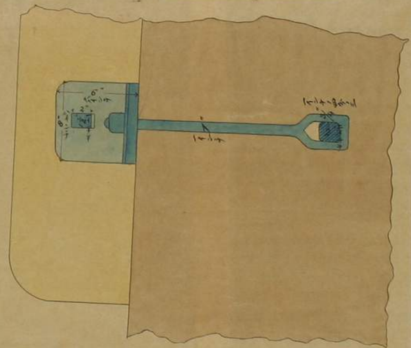
底ノ木防衝 FENDERS AT BOTTOM
