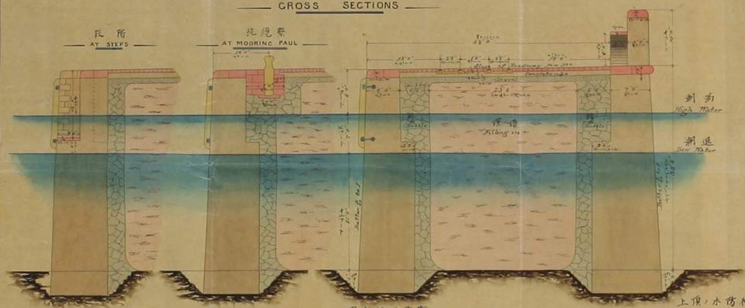
圖概橫 CROSS SECTIONS
